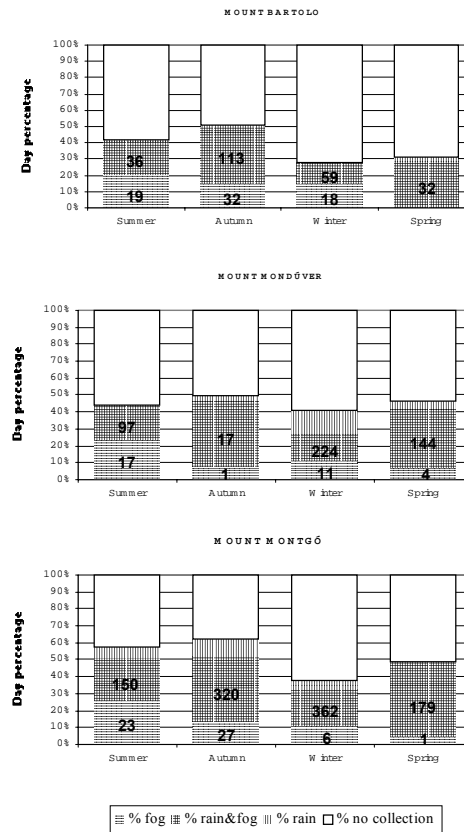
Figure 3. Seasonal percentage of days with only fog, fog and rainfall, and only rainfall collection.
