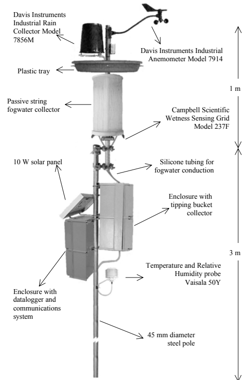
Figure 2. Integrated system for fog water collection and meteorological measurements
